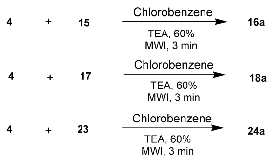
Scheme 9.
