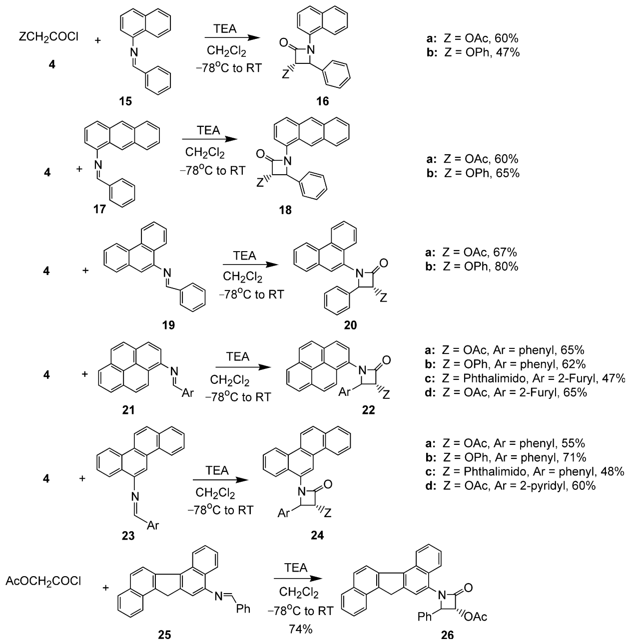
Scheme 5.
